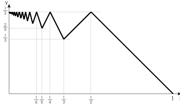
FIGURE 4. The “zigzag” function f .
